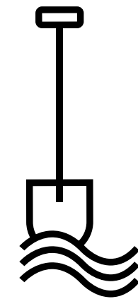
Bodem/ water
